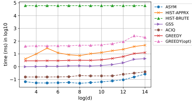
Figure 2: Average time per row spent on 4-bit quantization. Time is shown in log10 scale.
